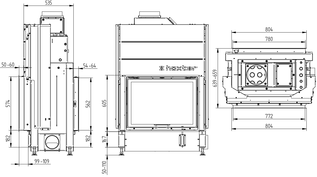
Cover frame 78/57h liftdoor 4sides 80 mm 1 x 90°
